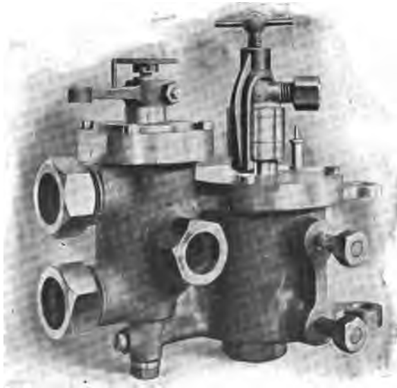
FIG. 322.—A Typical Float Feed Carburettor. This cut gives an outside elevation of the instrument shown in section in Fig. 282.
